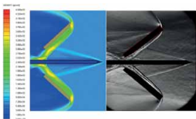
Sabot separation at muzzle exit: simulation (left) and experiment (right)
