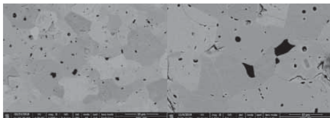
30-mm diameter (left) and 60-mm diameter (right) samples of \text{SiC} -doped \text{TiB}_2
