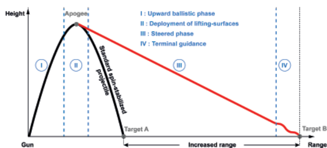
Flight phases of the long-range guided projectile
