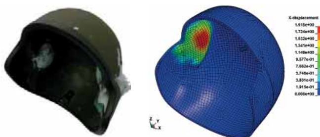
Experiment (left) and numerical simulation (right) to characterise a back face deformation
