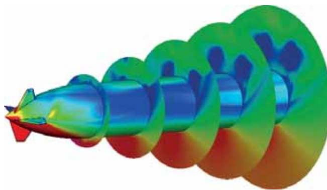
Simulation of the flow around the decoupled fuze guided projectile
