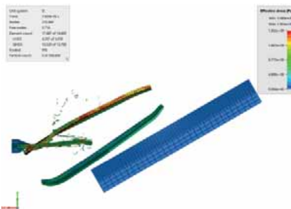
Numerical simulation to optimise the effectiveness of ERA plates
