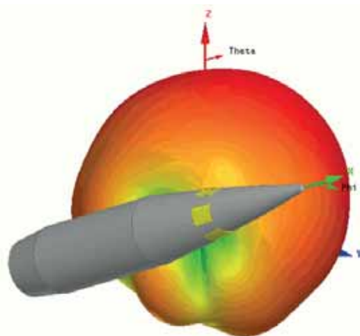
Roll-decoupled 3D radiation pattern associated to a GNSS antenna array
