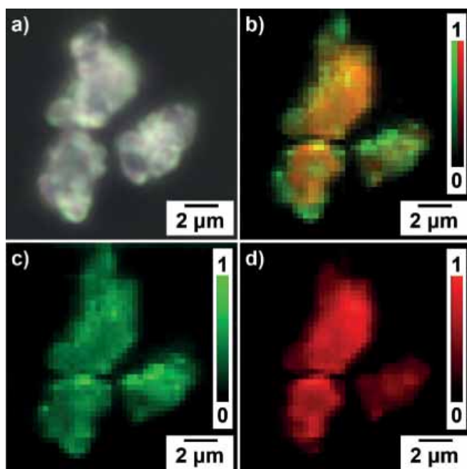
Hexolite nanoparticles
